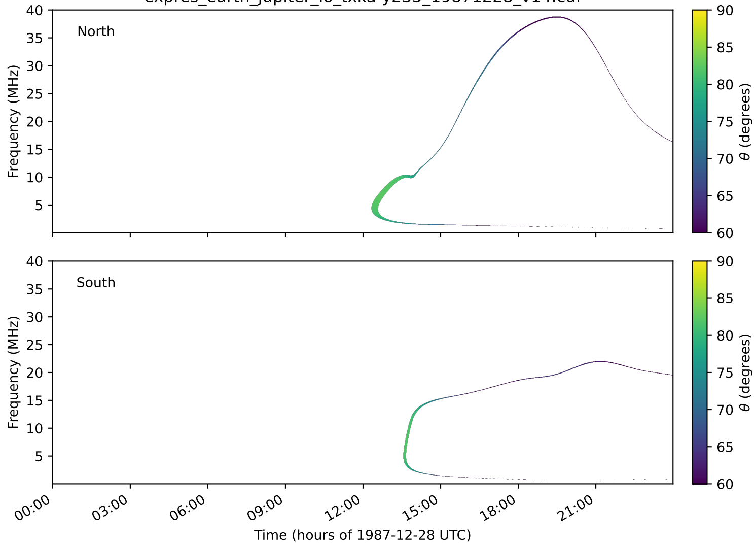
expres_earth_jupiter_io_txka-y235_19871228_v14.cdf
