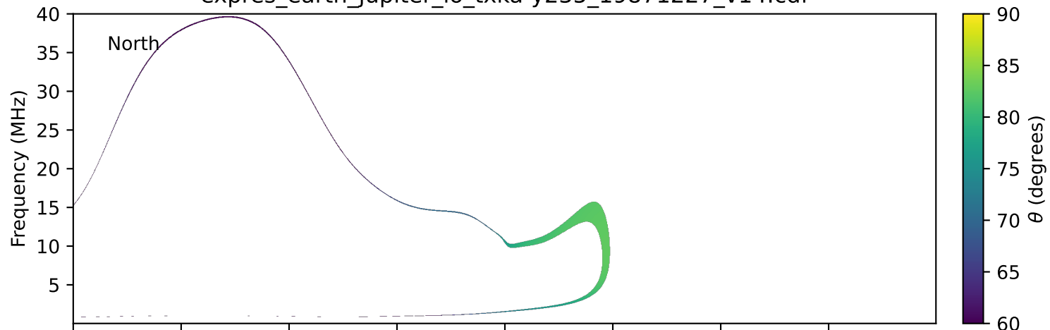
expres_earth_jupiter_io_txka-y235_19871227_v14.cdf
