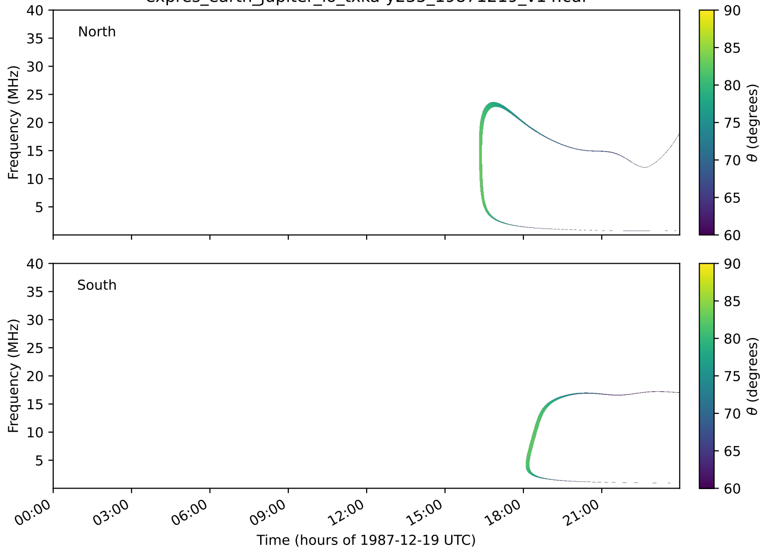
expres_earth_jupiter_io_txka-y235_19871219_v14.cdf
