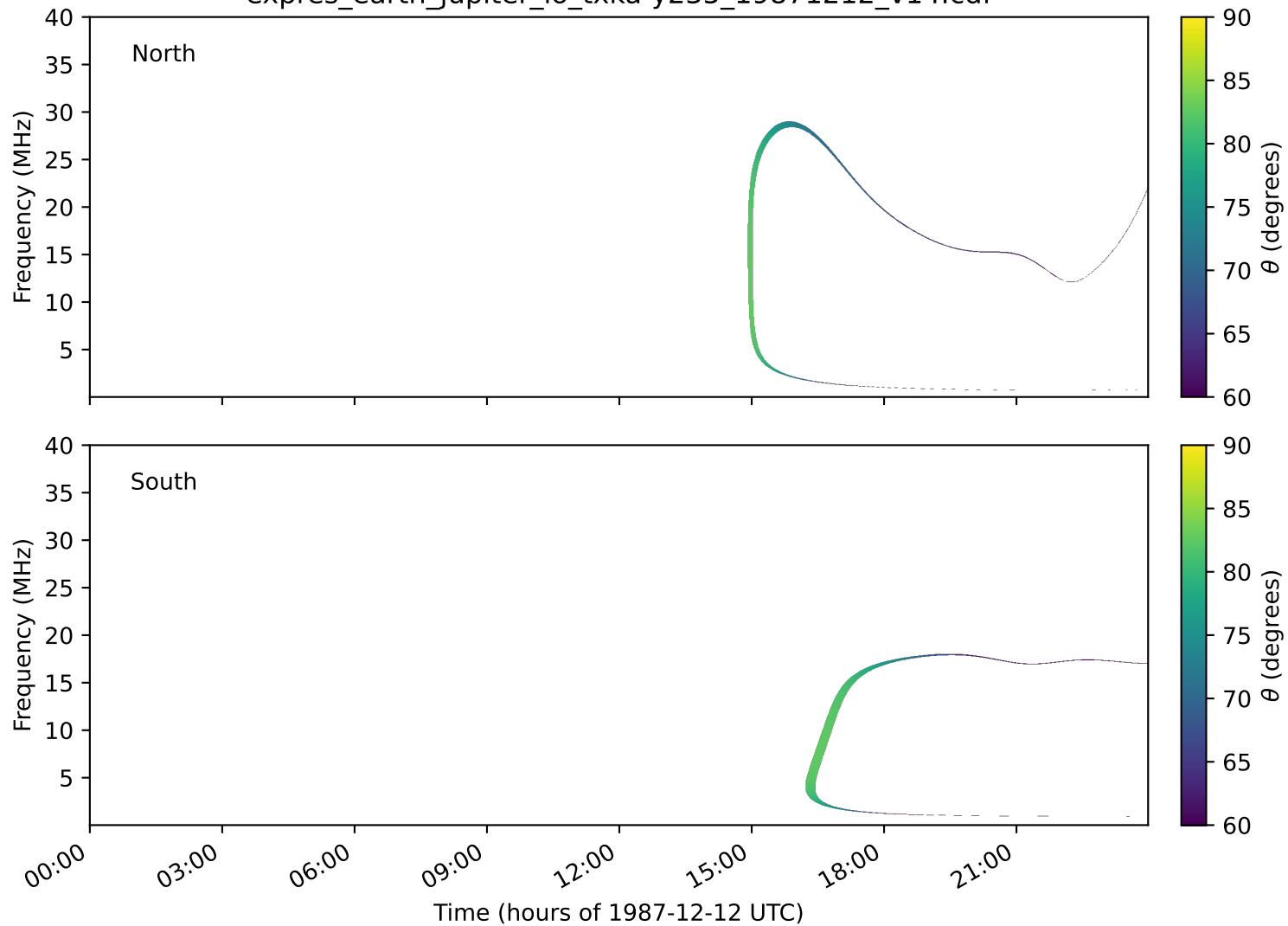
expres_earth_jupiter_io_txka-y235_19871212_v14.cdf
