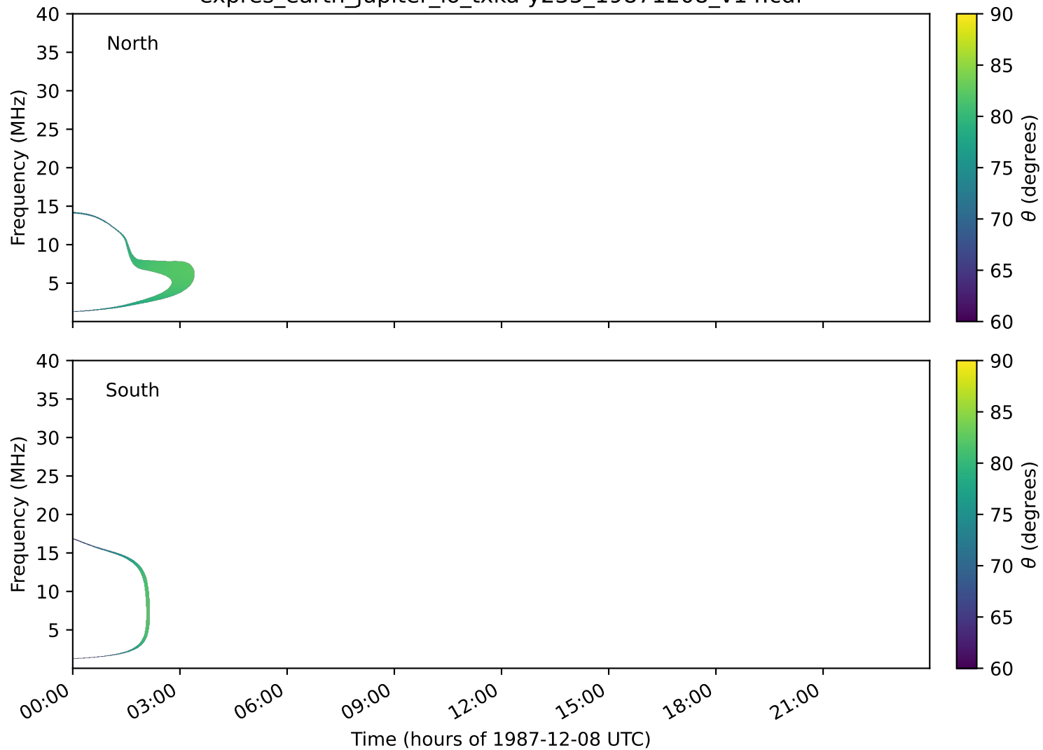
expres_earth_jupiter_io_txka-y235_19871208_v14.cdf
