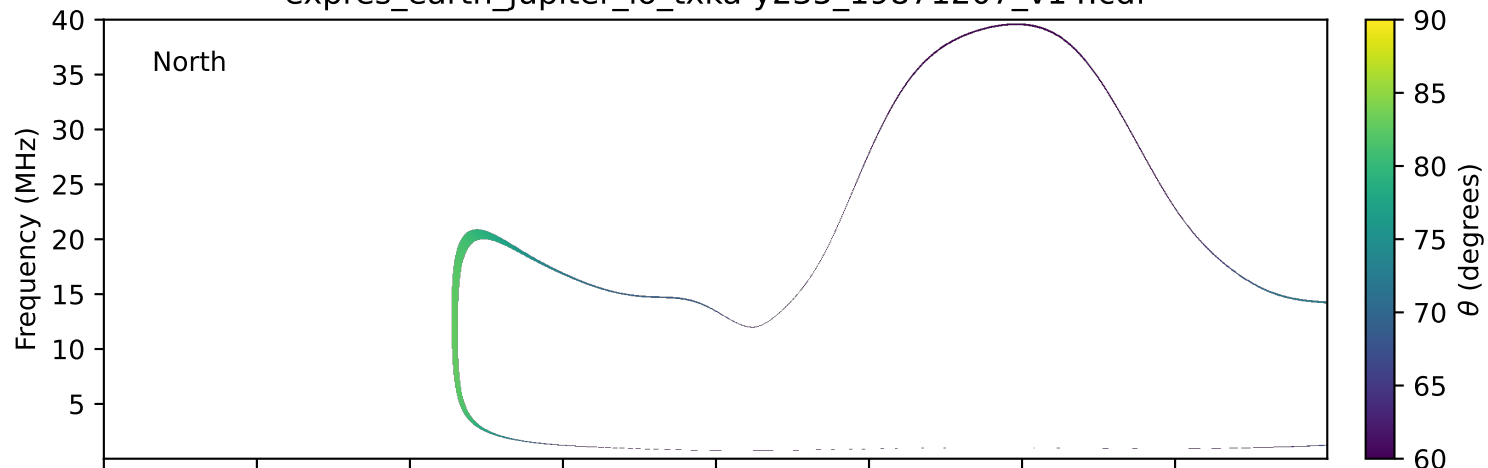
expres_earth_jupiter_io_txka-y235_19871207_v14.cdf
