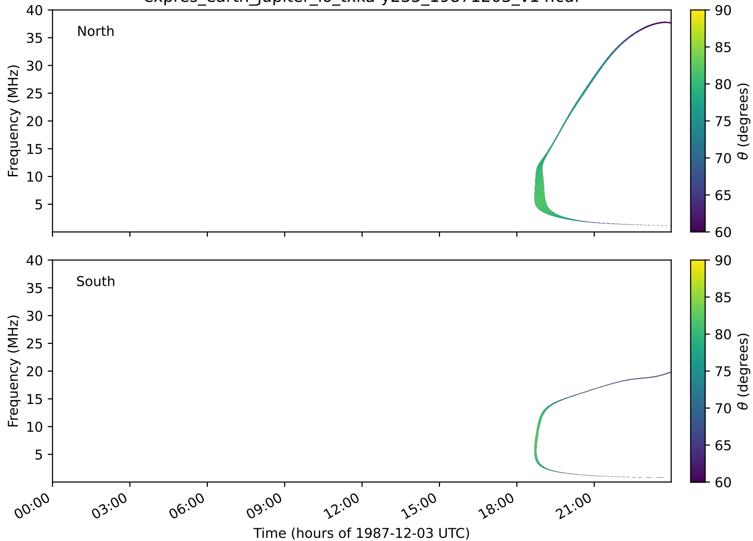
expres_earth_jupiter_io_txka-y235_19871203_v14.cdf
