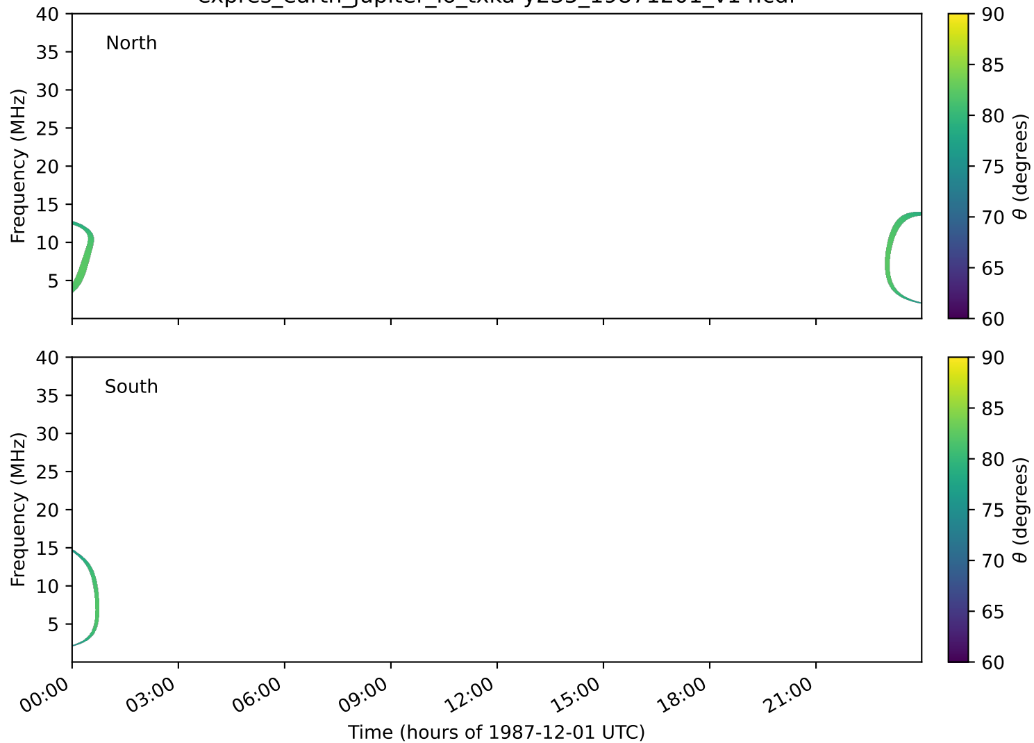
expres_earth_jupiter_io_txka-y235_19871201_v14.cdf
