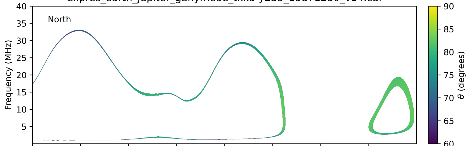
expres_earth_jupiter_ganymede_txka-y235_19871230_v14.cdf
