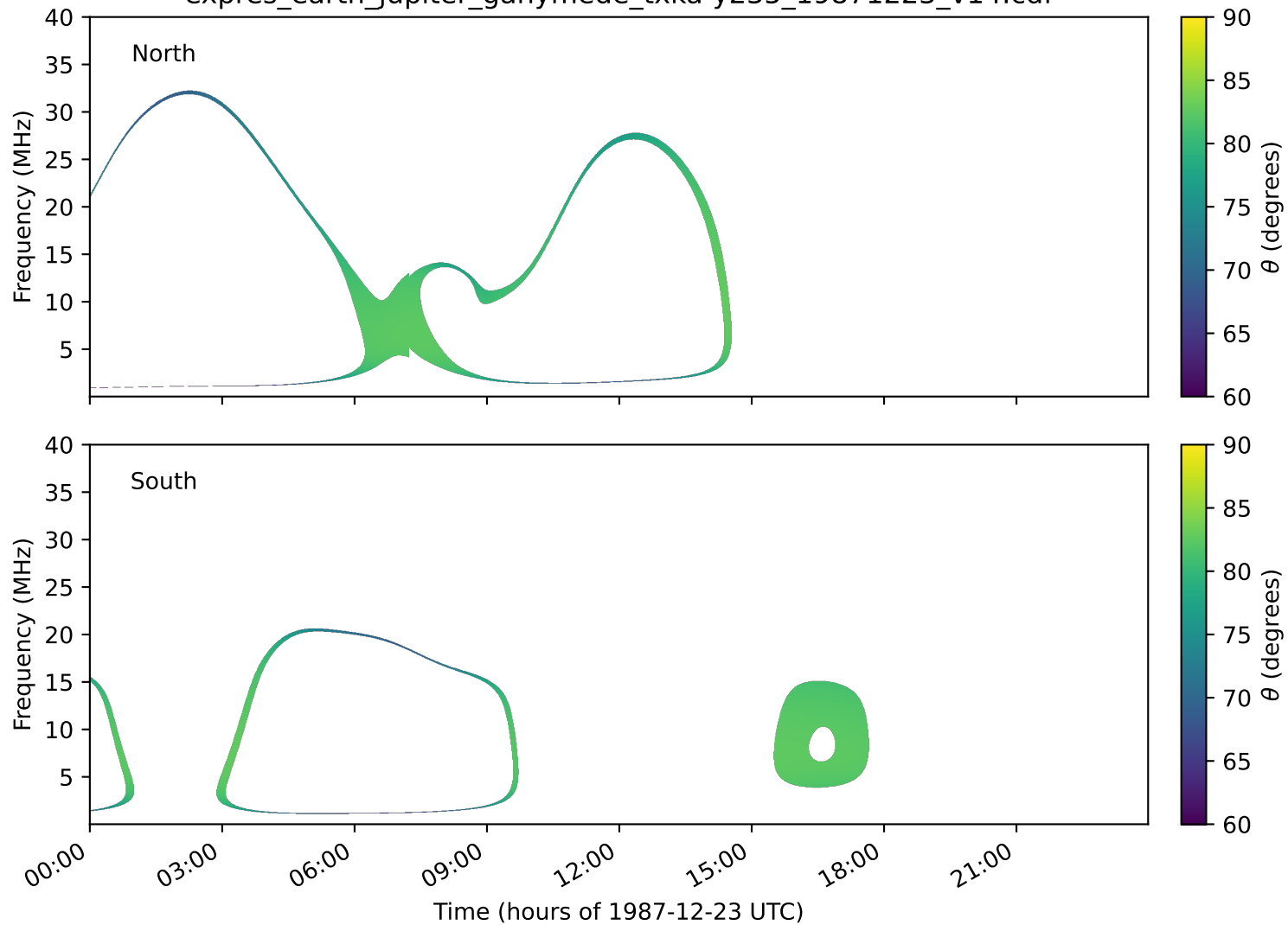
expres_earth_jupiter_ganymede_txka-y235_19871223_v14.cdf
