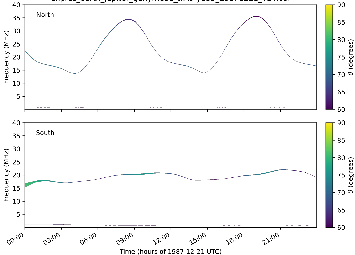
expres_earth_jupiter_ganymede_txka-y235_19871221_v14.cdf
