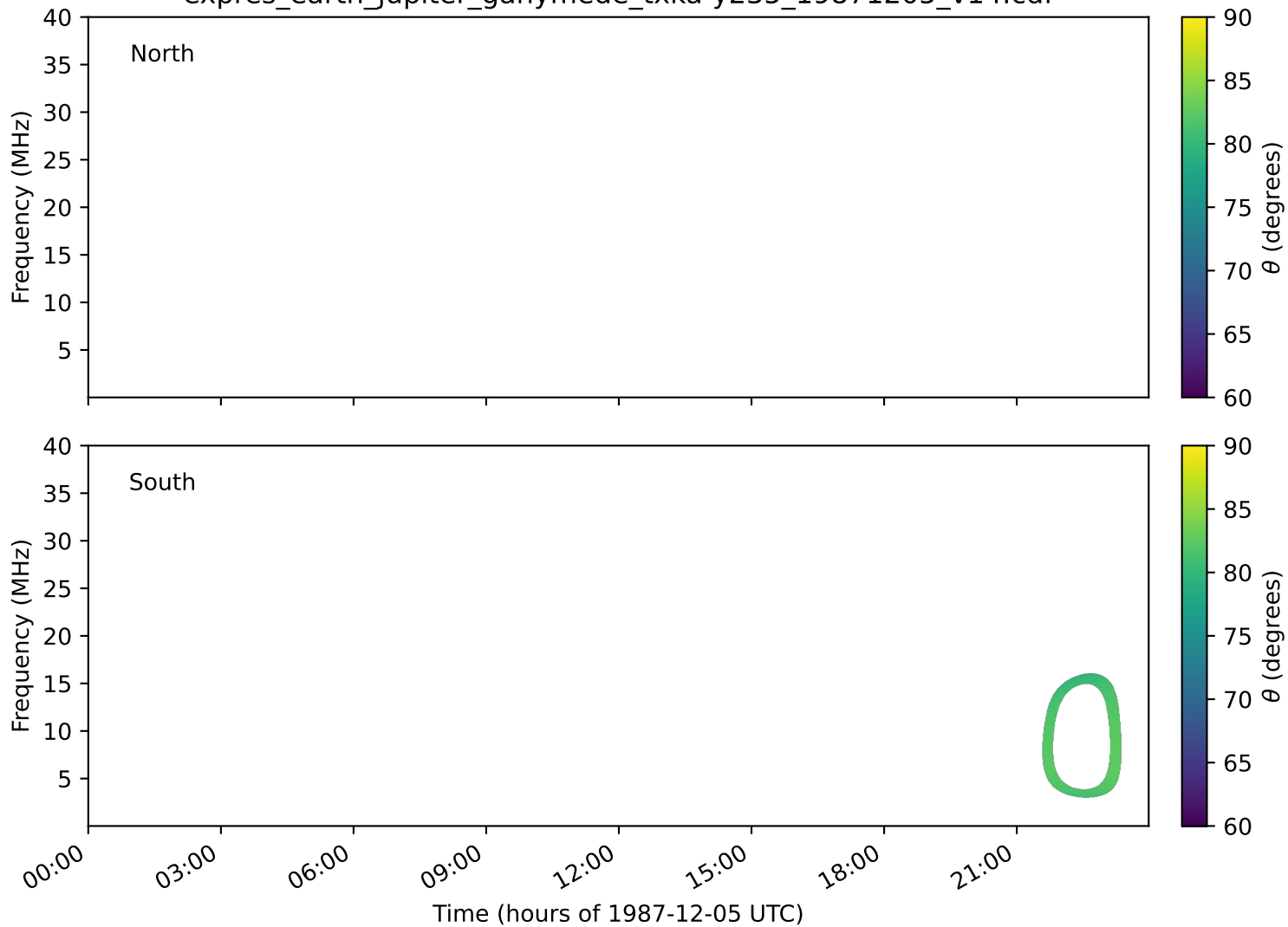
expres_earth_jupiter_ganymede_txka-y235_19871205_v14.cdf
