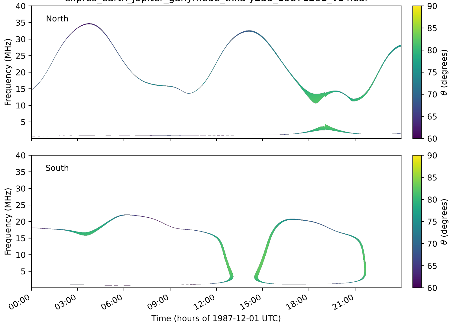
expres_earth_jupiter_ganymede_txka-y235_19871201_v14.cdf
