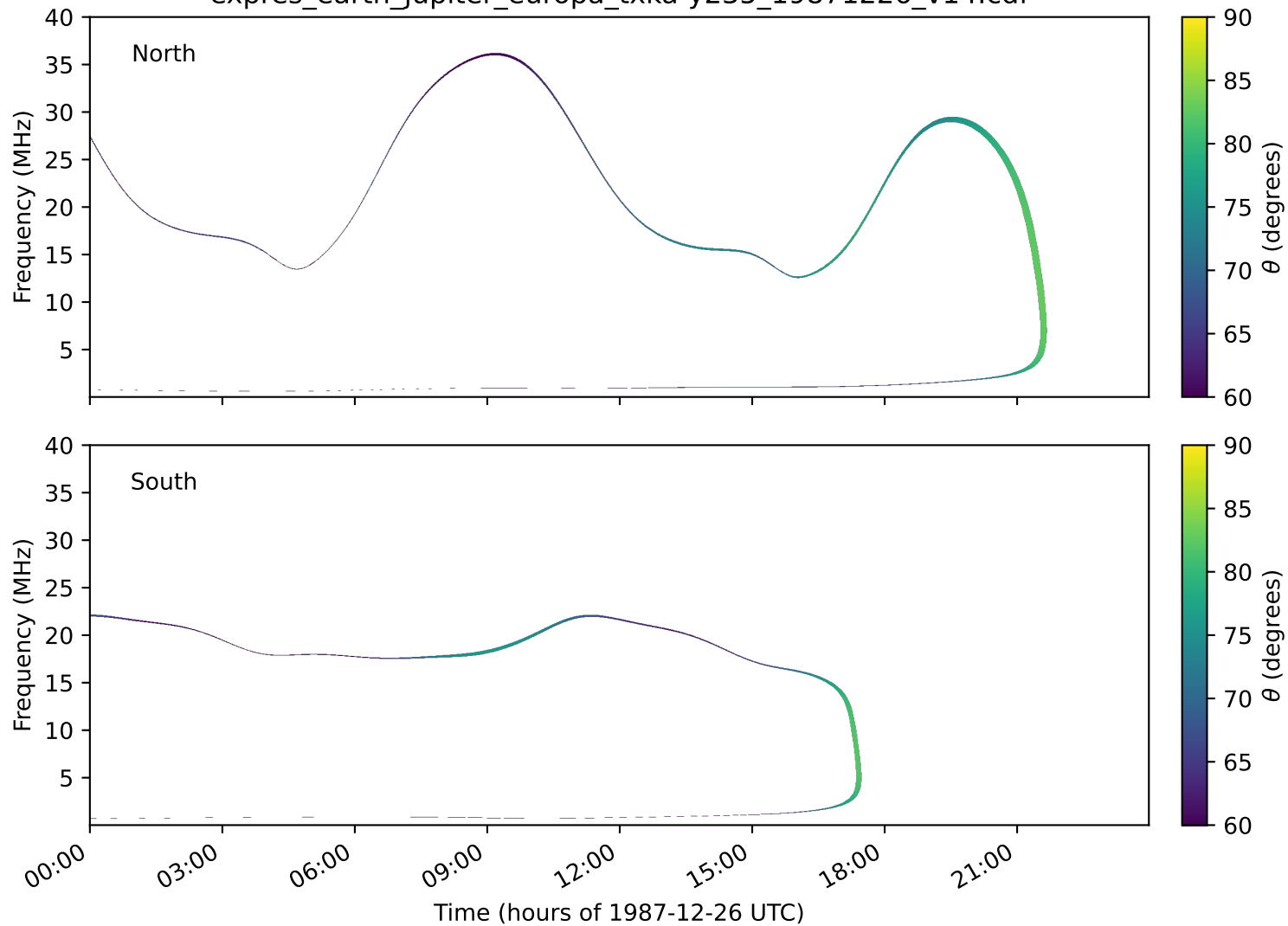
expres_earth_jupiter_europa_txka-y235_19871226_v14.cdf
