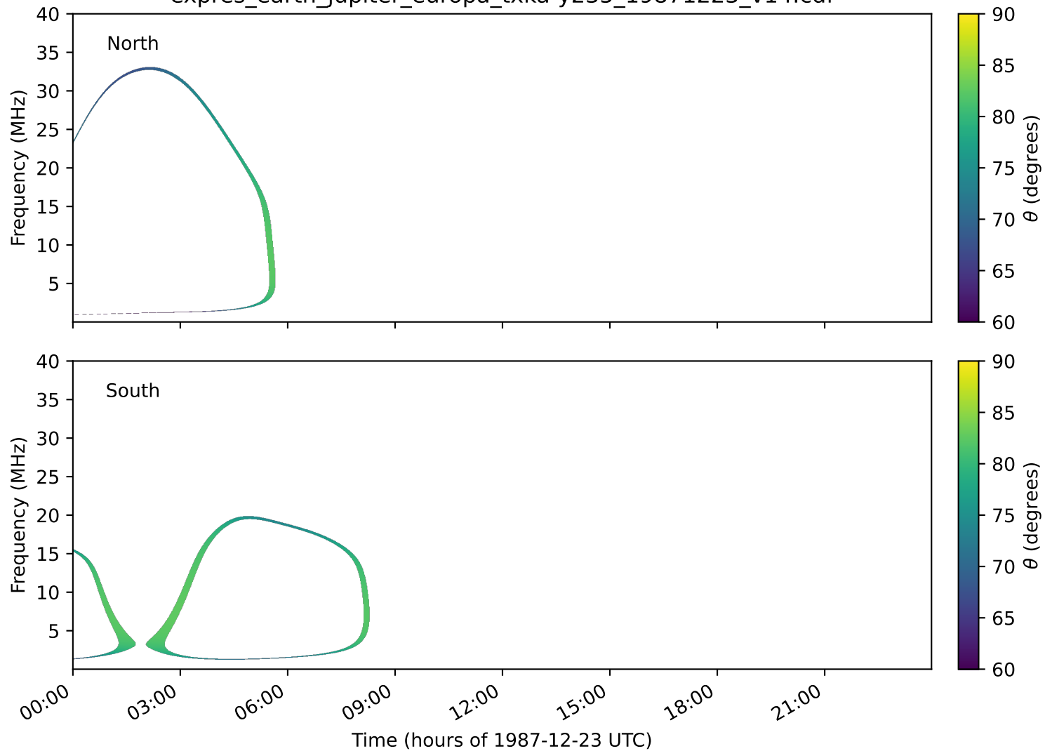
expres_earth_jupiter_europa_txka-y235_19871223_v14.cdf
