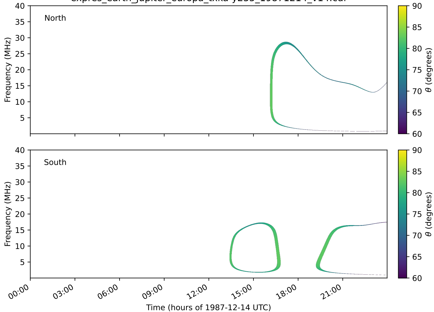
expres_earth_jupiter_europa_txka-y235_19871214_v14.cdf
