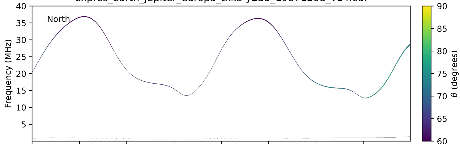
expres_earth_jupiter_europa_txka-y235_19871208_v14.cdf
