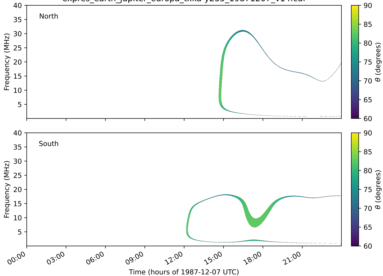
expres_earth_jupiter_europa_txka-y235_19871207_v14.cdf
