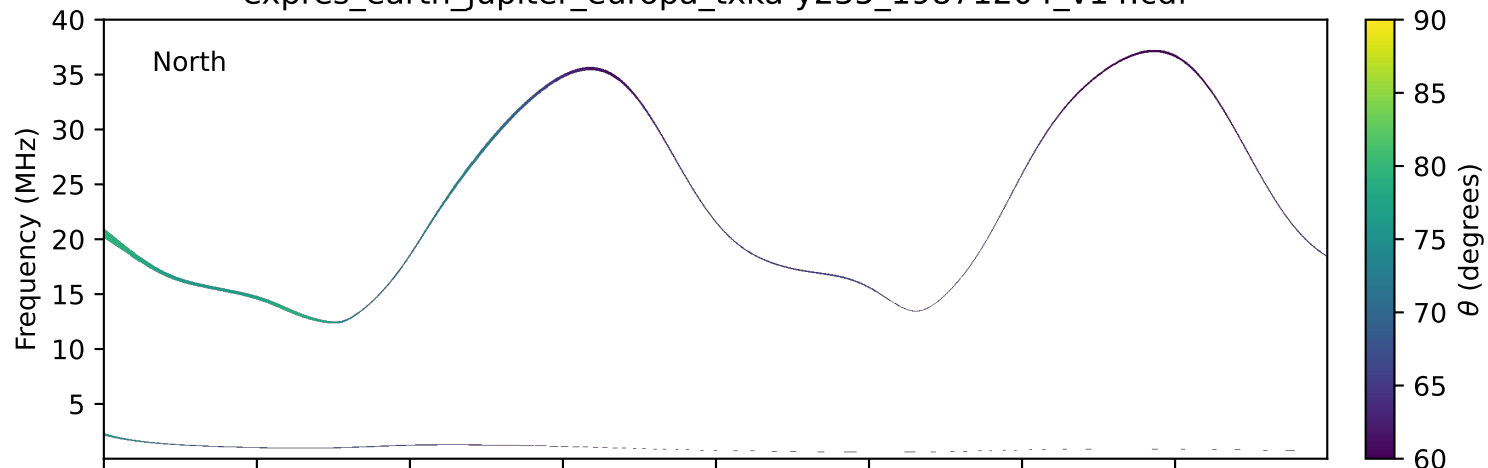
expres_earth_jupiter_europa_txka-y235_19871204_v14.cdf
