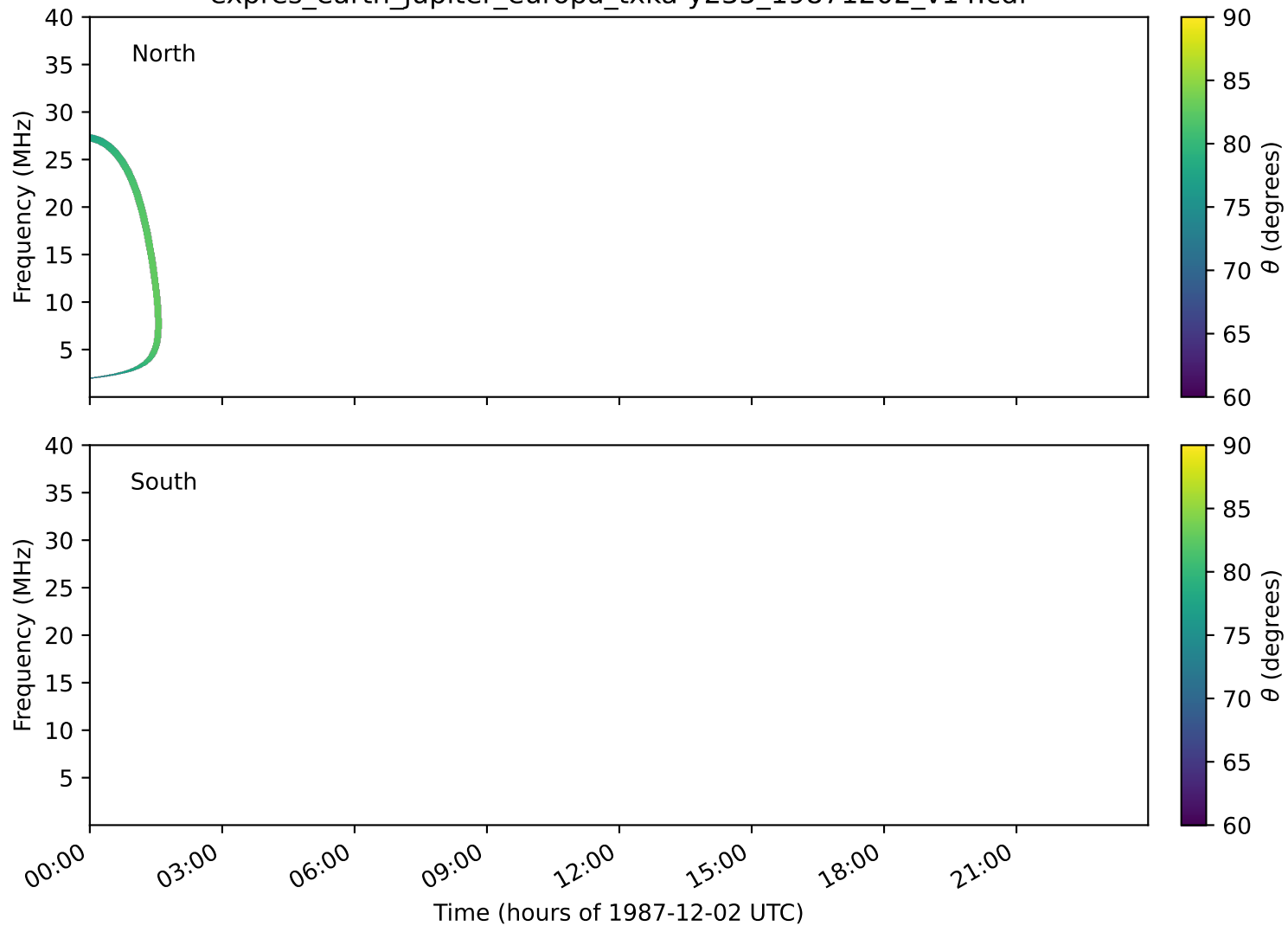
expres_earth_jupiter_europa_txka-y235_19871202_v14.cdf
