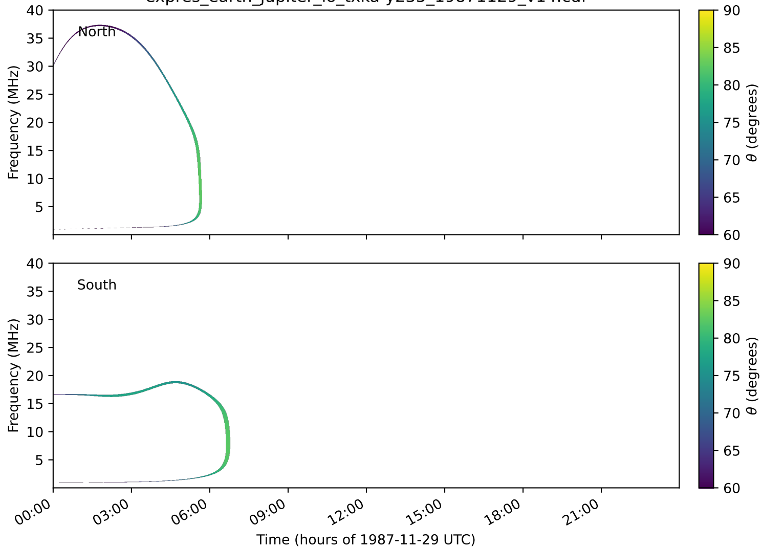
expres_earth_jupiter_io_txka-y235_19871129_v14.cdf
