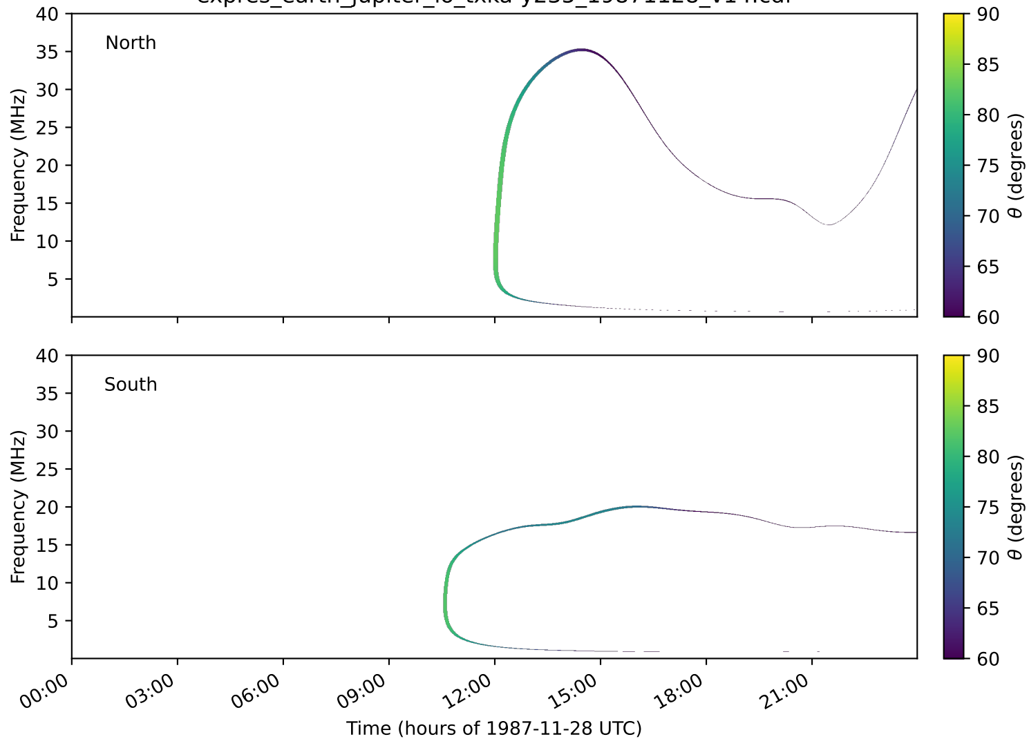
expres_earth_jupiter_io_txka-y235_19871128_v14.cdf
