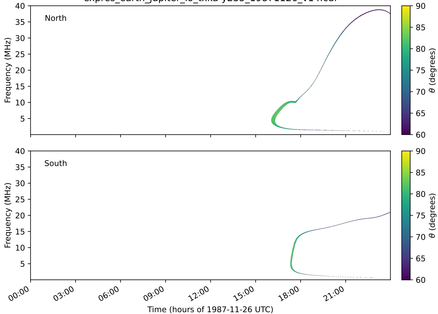
expres_earth_jupiter_io_txka-y235_19871126_v14.cdf
