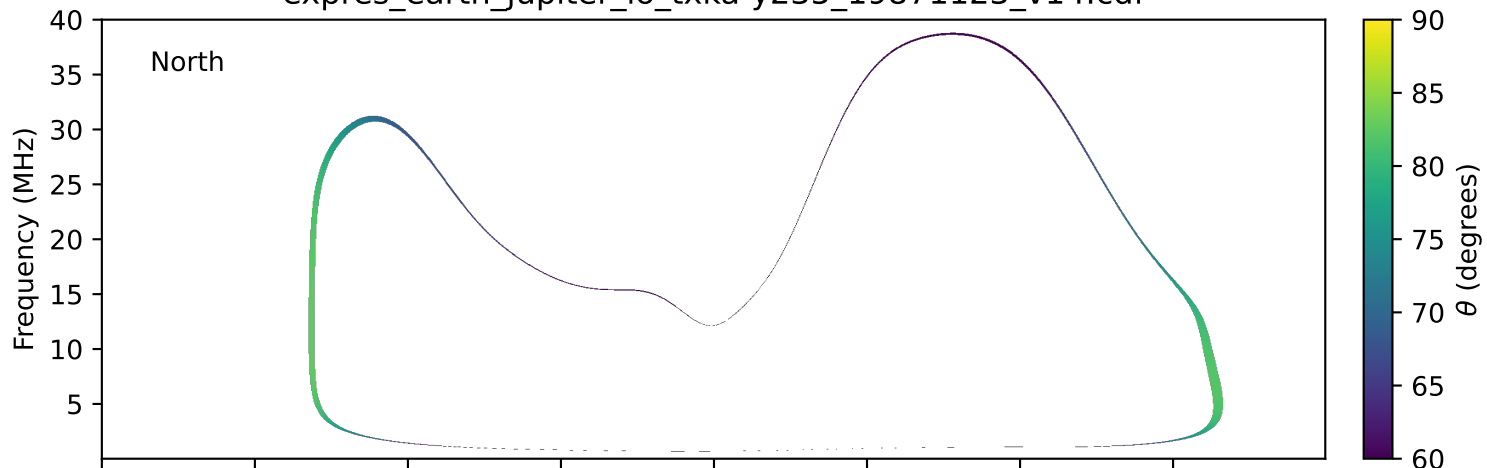
expres_earth_jupiter_io_txka-y235_19871123_v14.cdf
