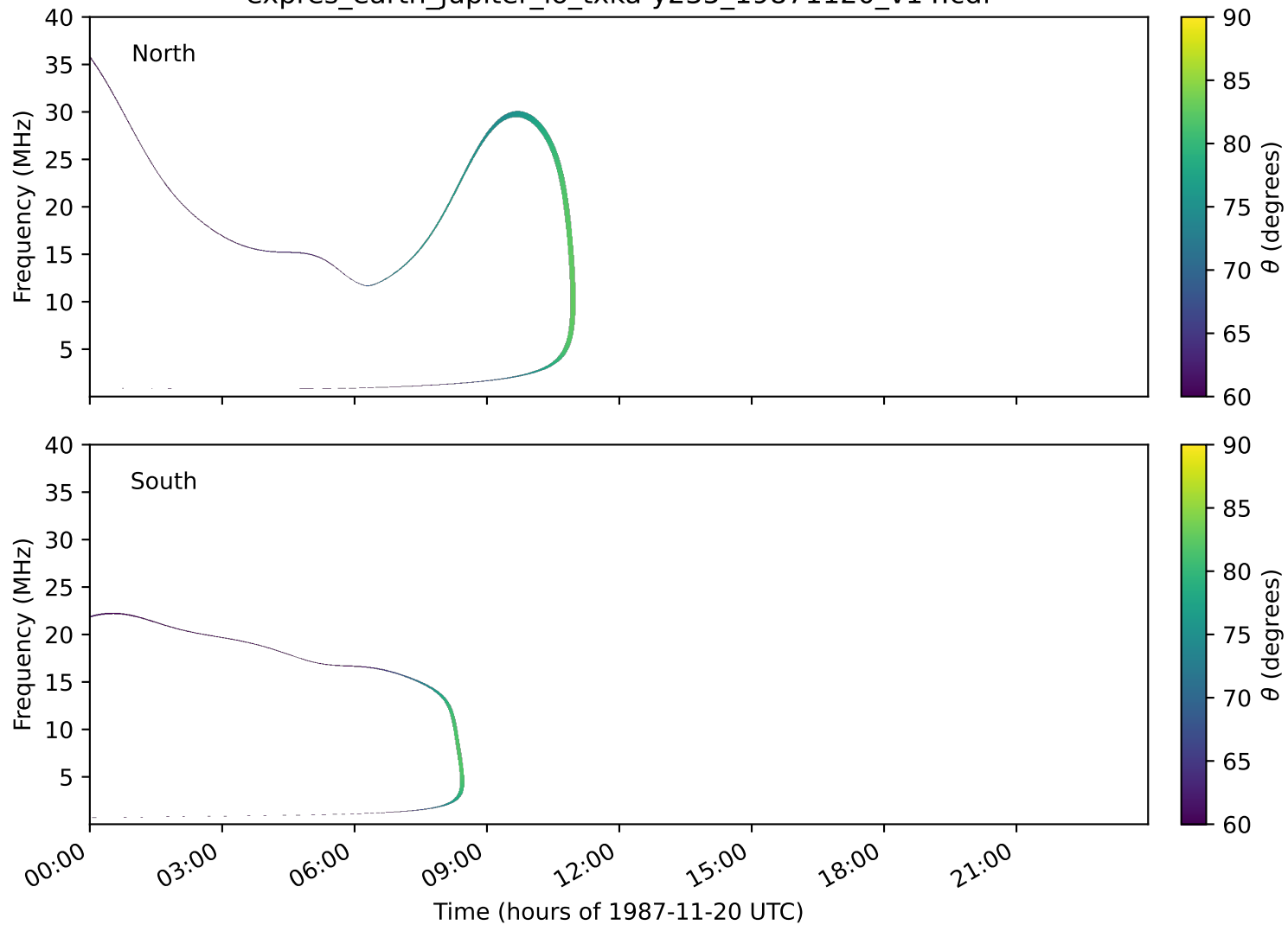
expres_earth_jupiter_io_txka-y235_19871120_v14.cdf
