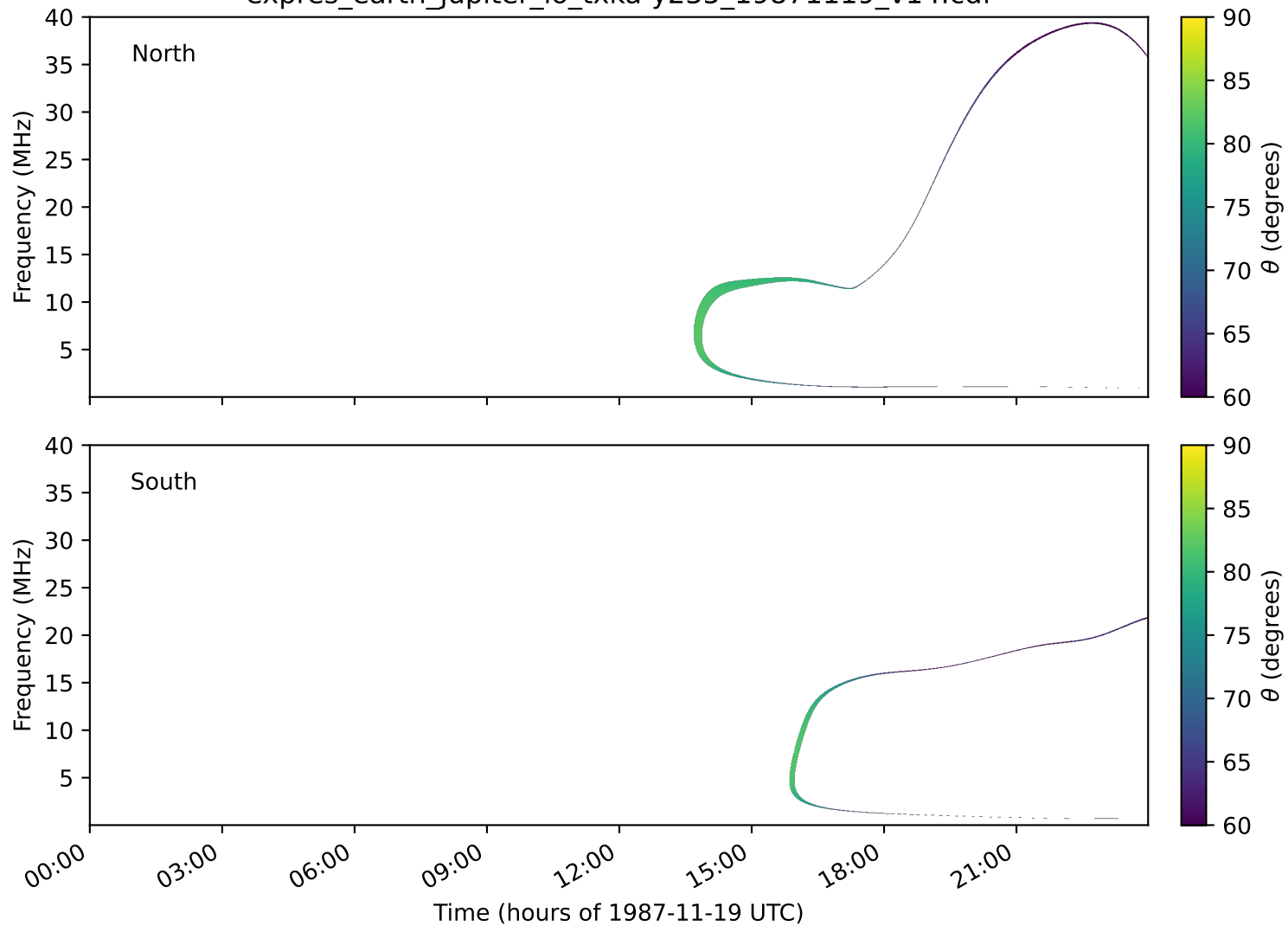
expres_earth_jupiter_io_txka-y235_19871119_v14.cdf
