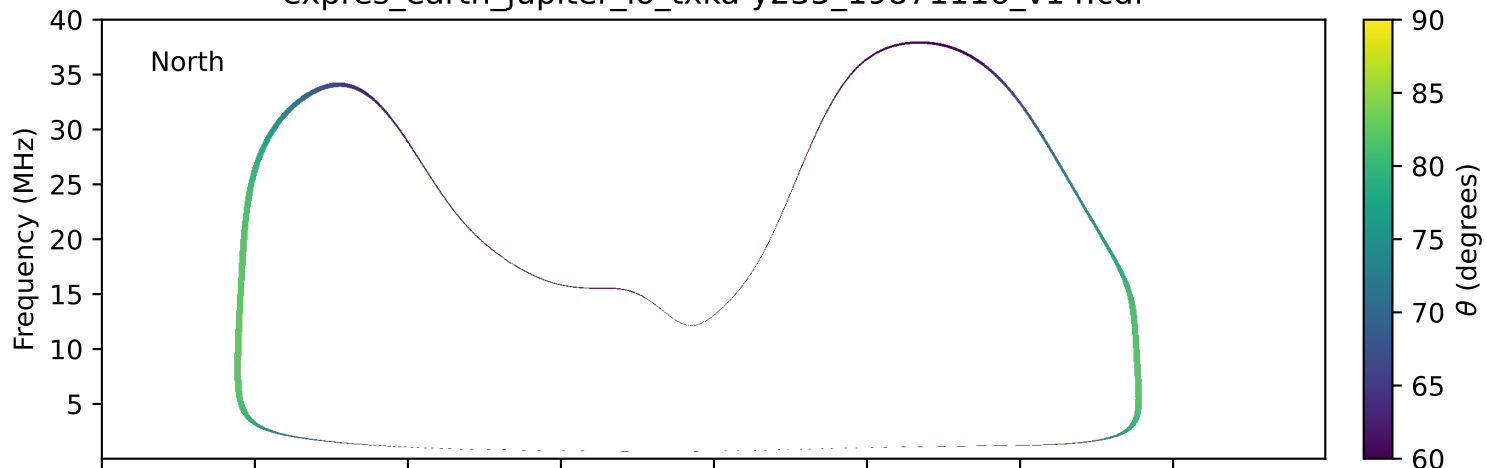
expres_earth_jupiter_io_txka-y235_19871116_v14.cdf
