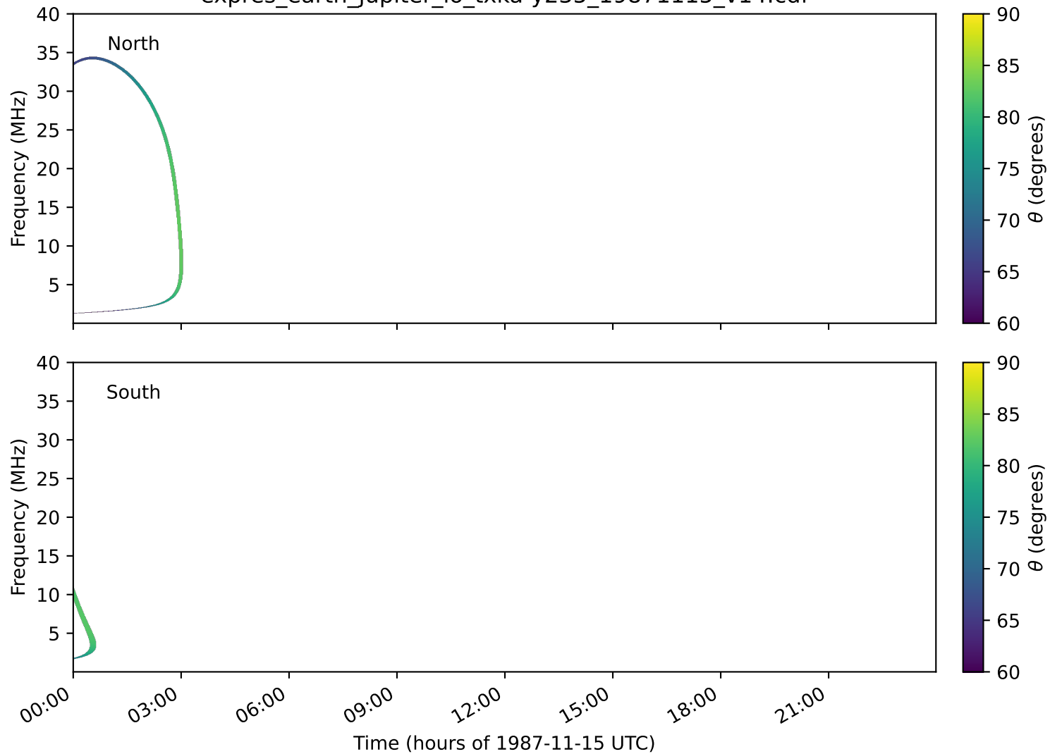
expres_earth_jupiter_io_txka-y235_19871115_v14.cdf
