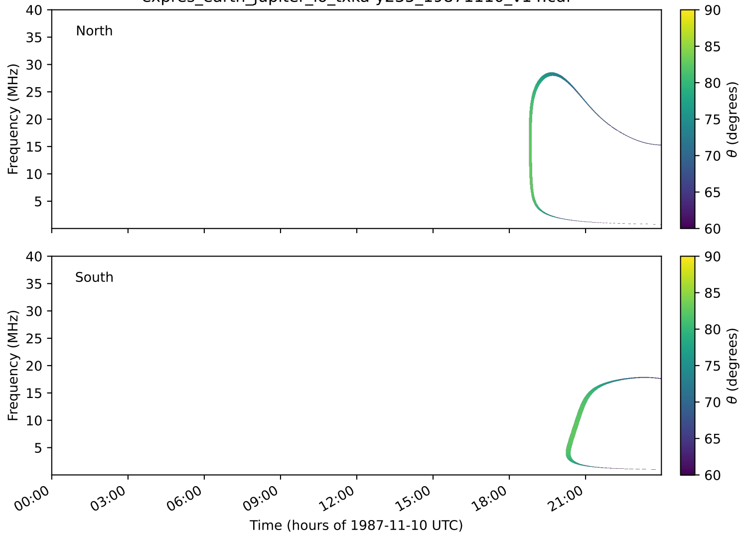
expres_earth_jupiter_io_txka-y235_19871110_v14.cdf
