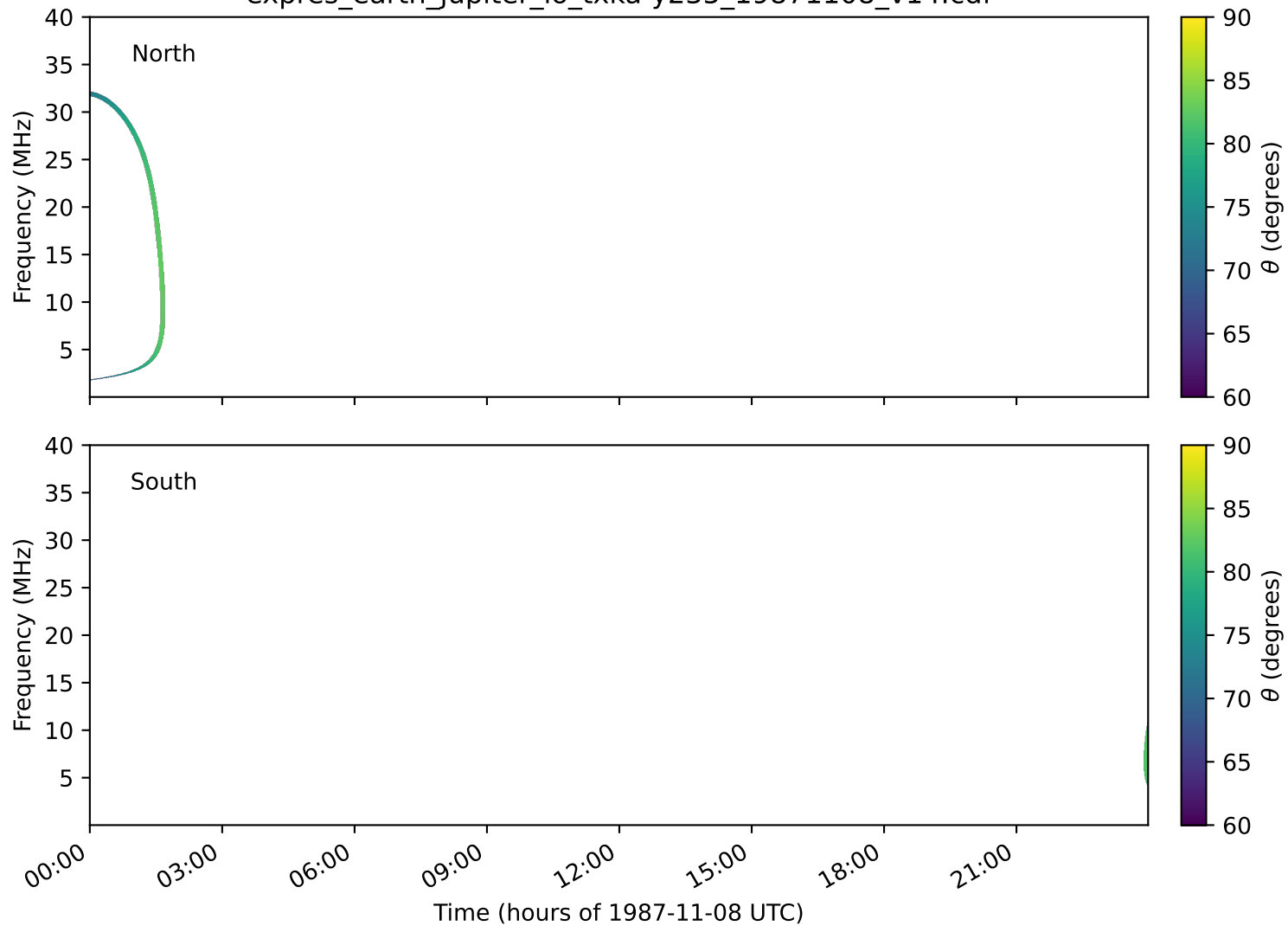
expres_earth_jupiter_io_txka-y235_19871108_v14.cdf
