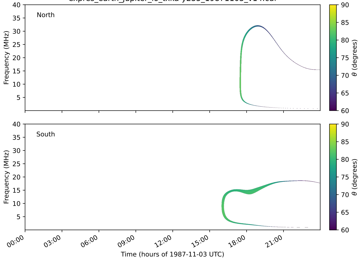
expres_earth_jupiter_io_txka-y235_19871103_v14.cdf
