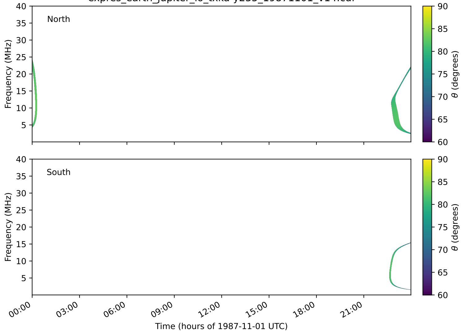
expres_earth_jupiter_io_txka-y235_19871101_v14.cdf
