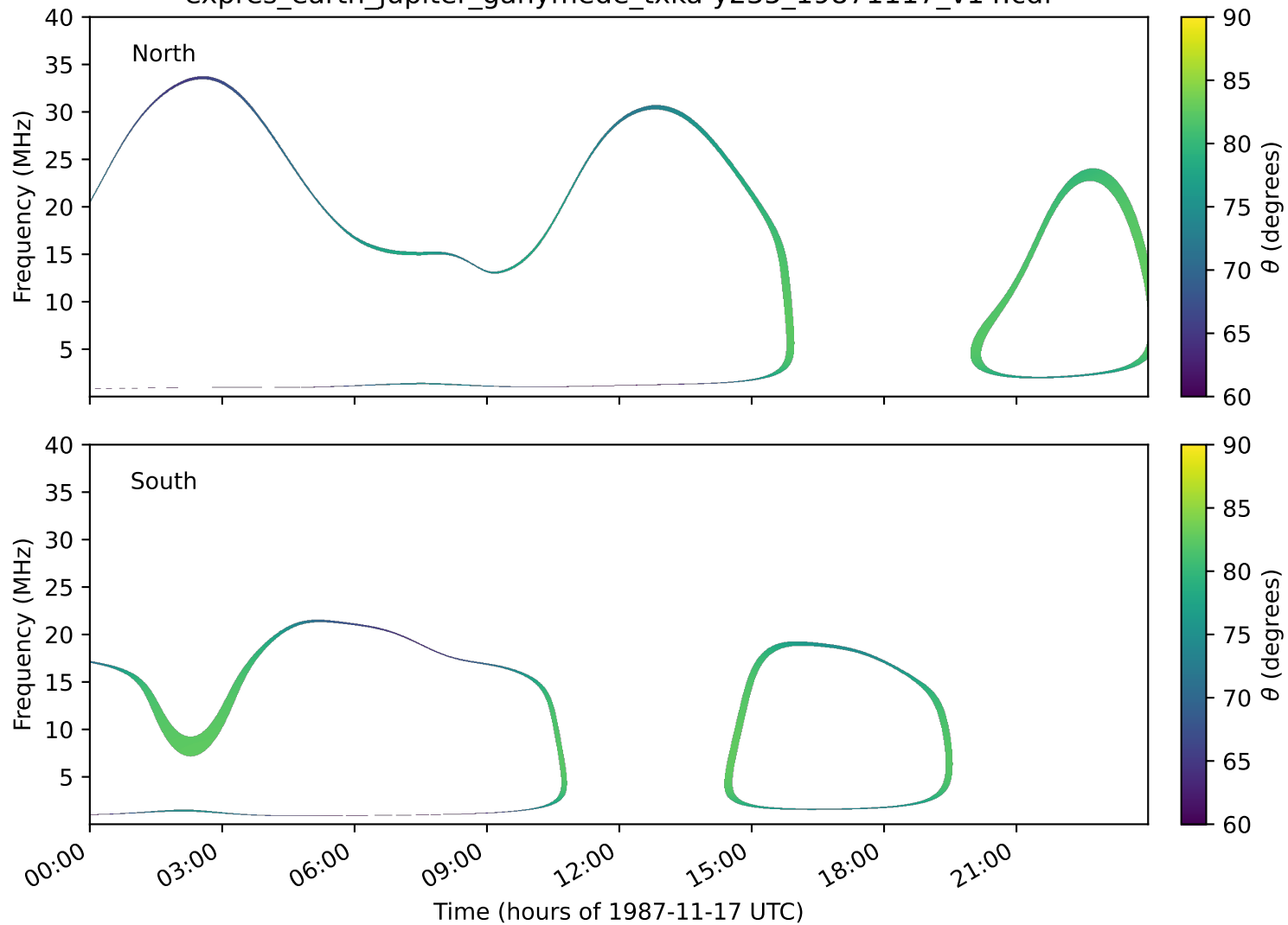
expres_earth_jupiter_ganymede_txka-y235_19871117_v14.cdf
