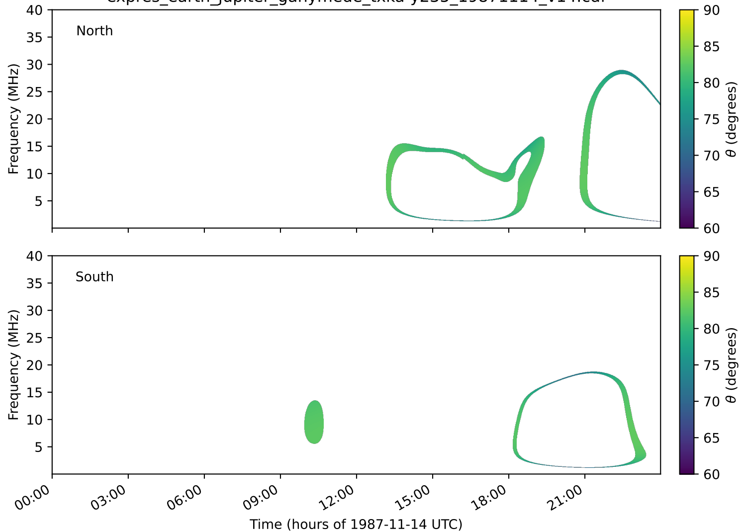
expres_earth_jupiter_ganymede_txka-y235_19871114_v14.cdf
