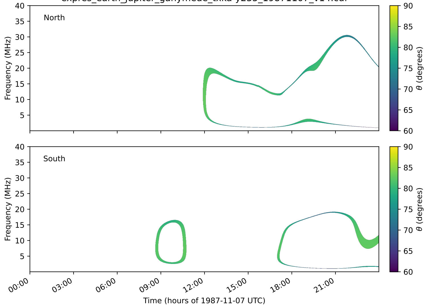
expres_earth_jupiter_ganymede_txka-y235_19871107_v14.cdf
