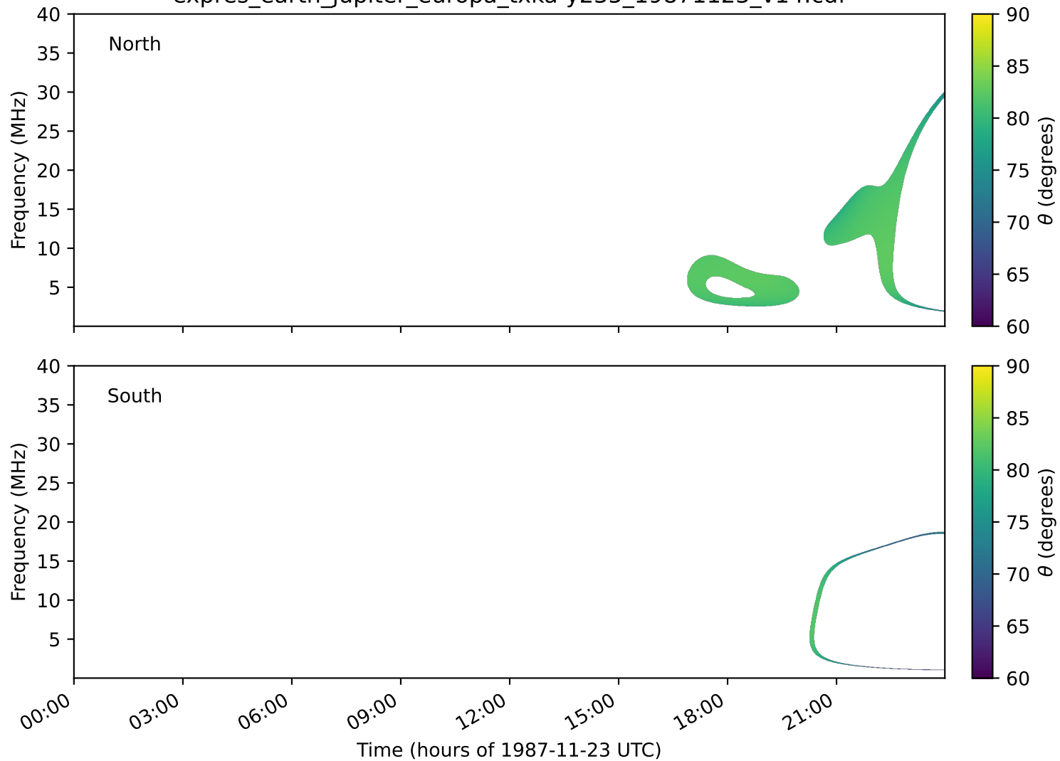
expres_earth_jupiter_europa_txka-y235_19871123_v14.cdf
