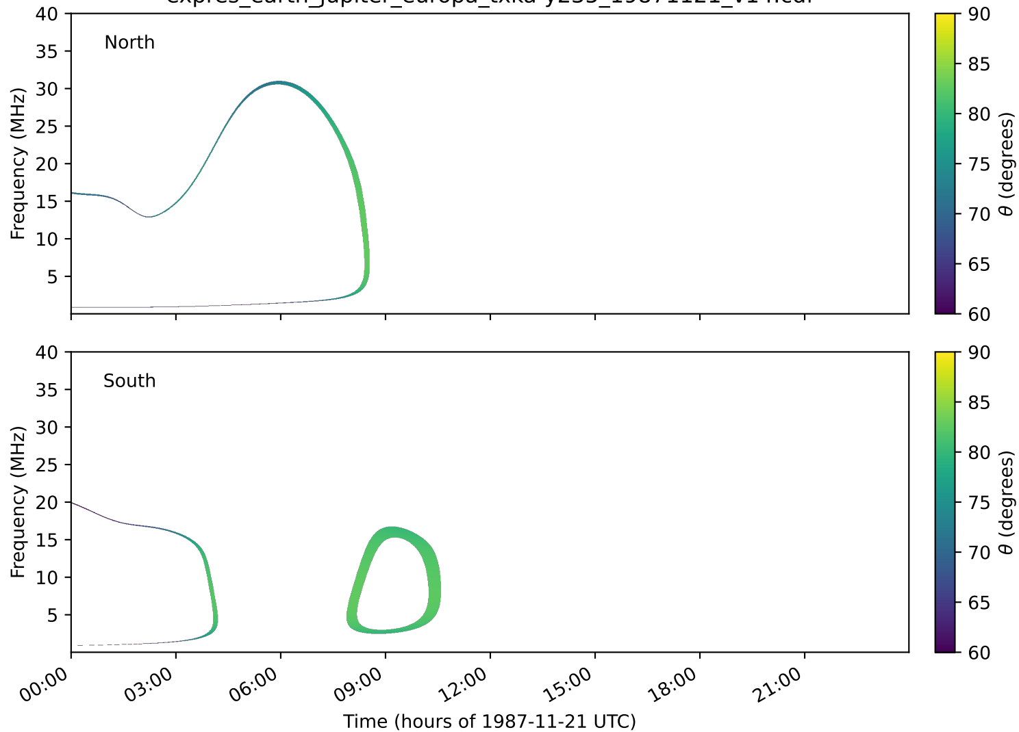
expres_earth_jupiter_europa_txka-y235_19871121_v14.cdf
