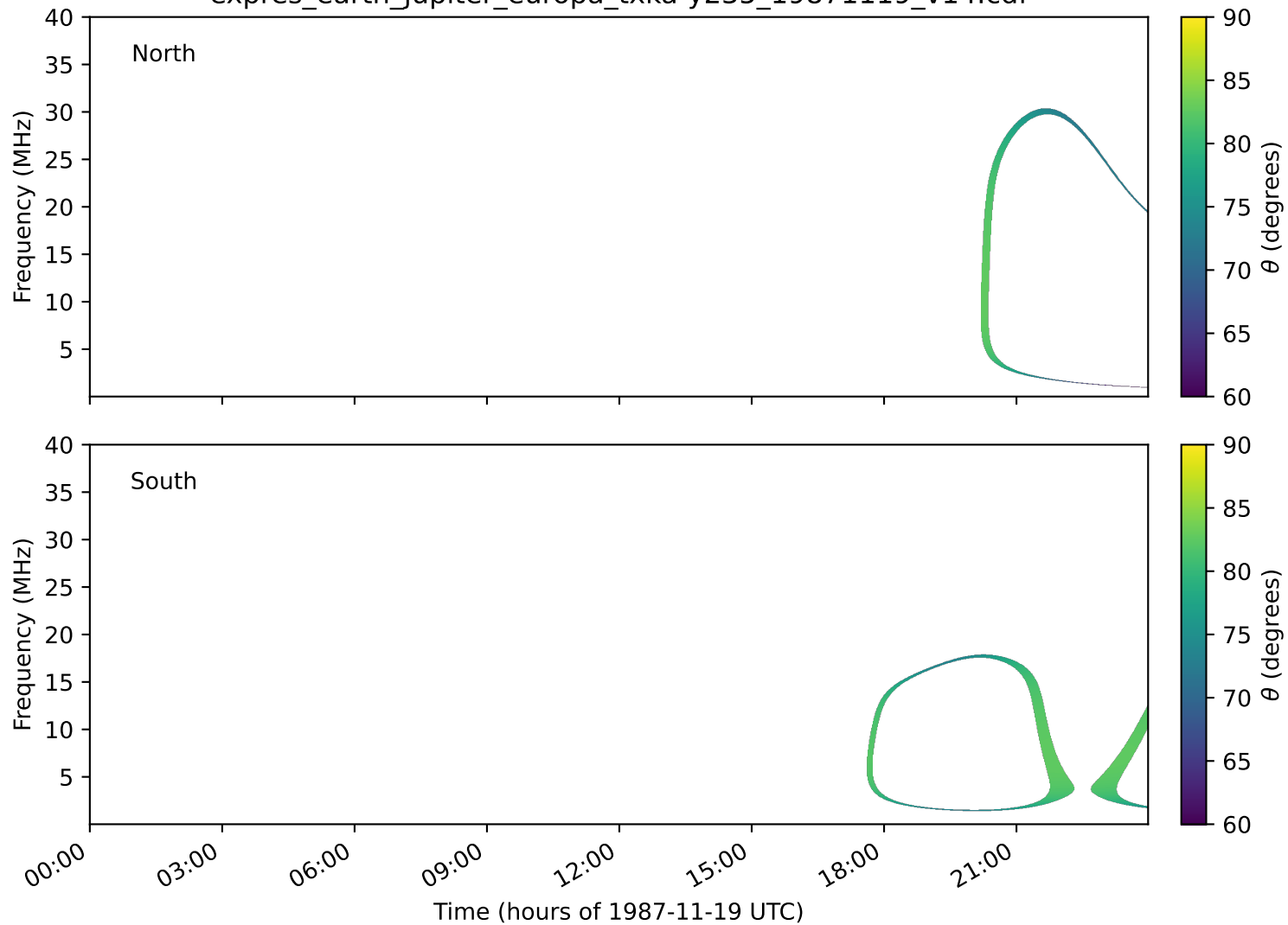
expres_earth_jupiter_europa_txka-y235_19871119_v14.cdf
