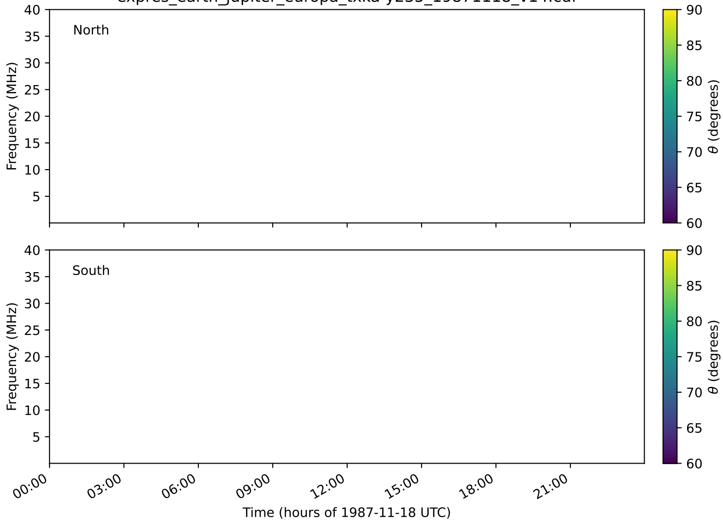
expres_earth_jupiter_europa_txka-y235_19871118_v14.cdf
