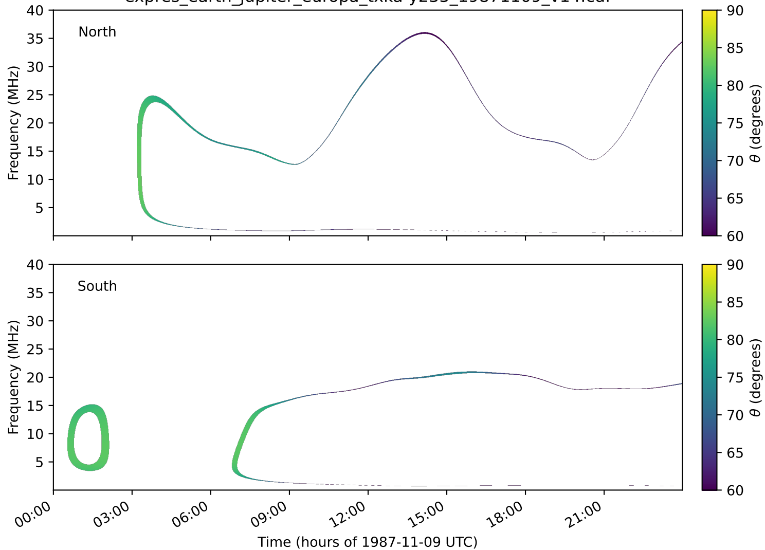
expres_earth_jupiter_europa_txka-y235_19871109_v14.cdf
