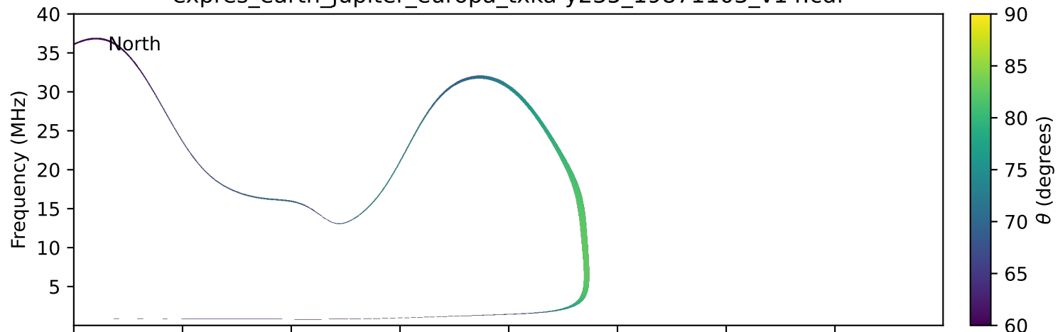
expres_earth_jupiter_europa_txka-y235_19871103_v14.cdf
