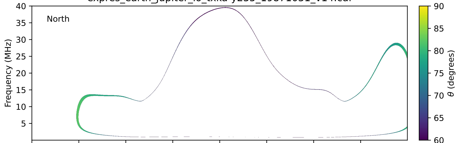
expres_earth_jupiter_io_txka-y235_19871031_v14.cdf
