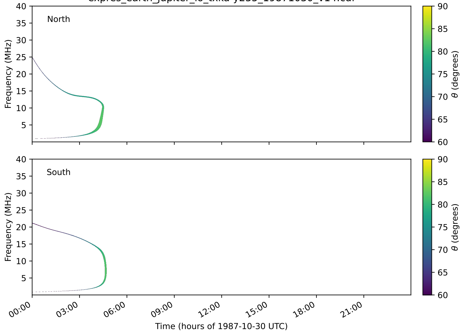
expres_earth_jupiter_io_txka-y235_19871030_v14.cdf
