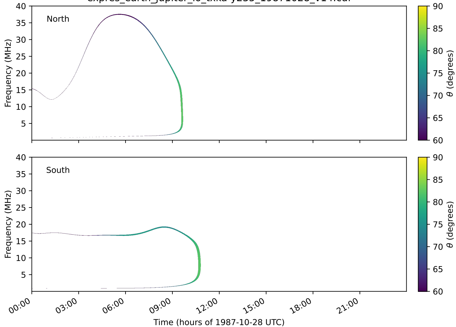
expres_earth_jupiter_io_txka-y235_19871028_v14.cdf
