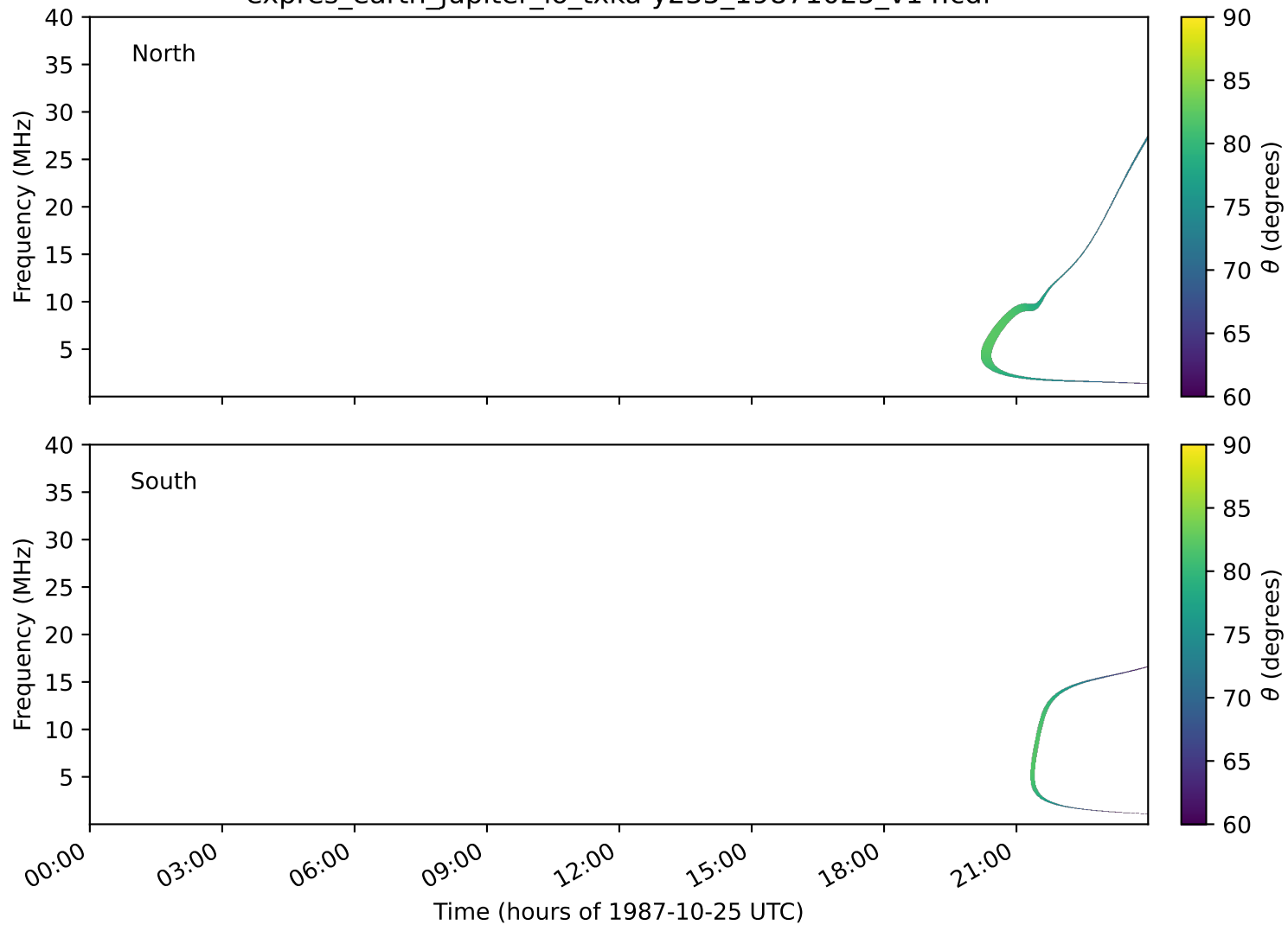
expres_earth_jupiter_io_txka-y235_19871025_v14.cdf
