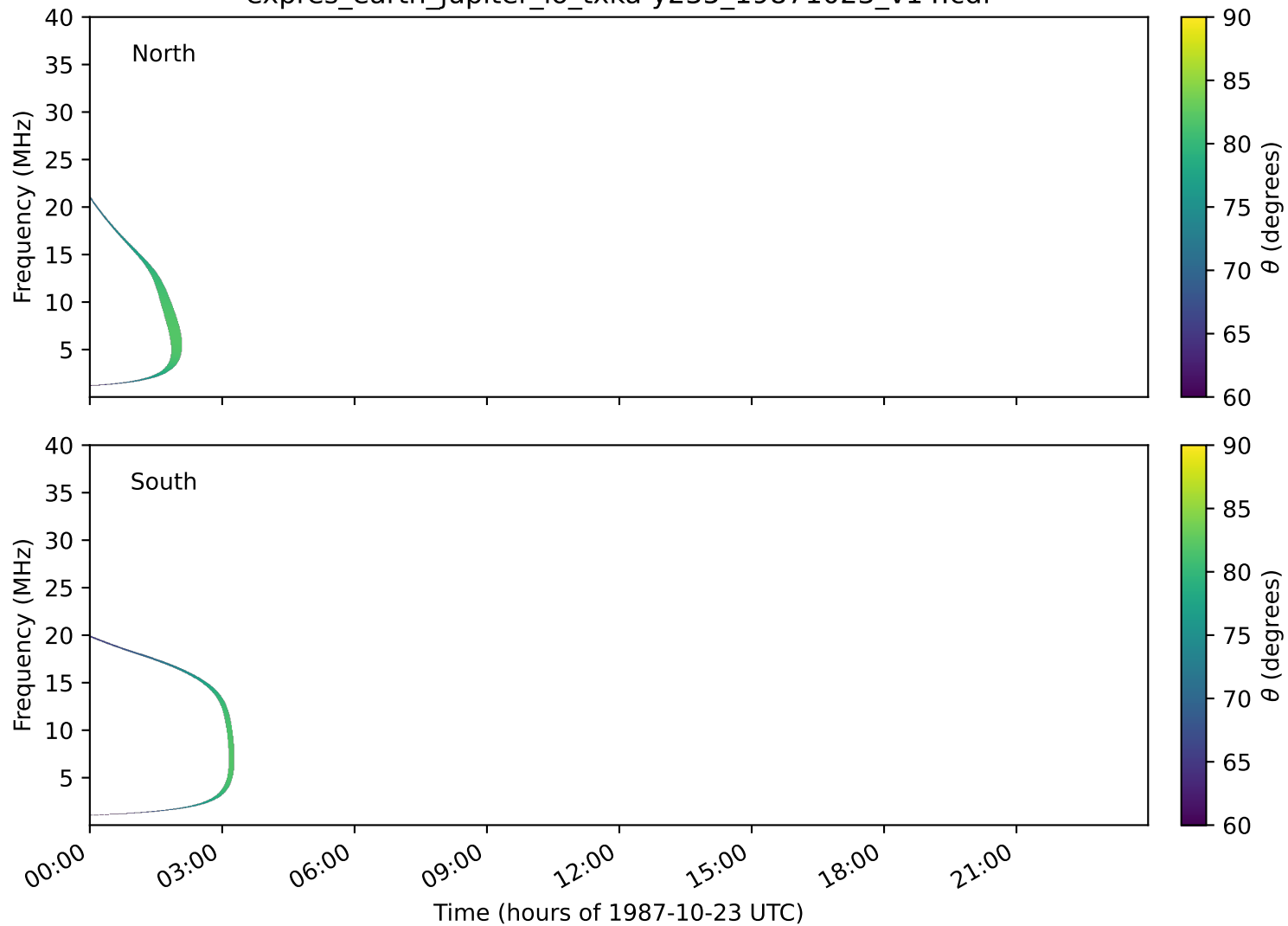
expres_earth_jupiter_io_txka-y235_19871023_v14.cdf
