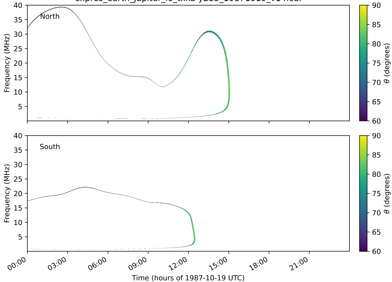
expres_earth_jupiter_io_txka-y235_19871019_v14.cdf
