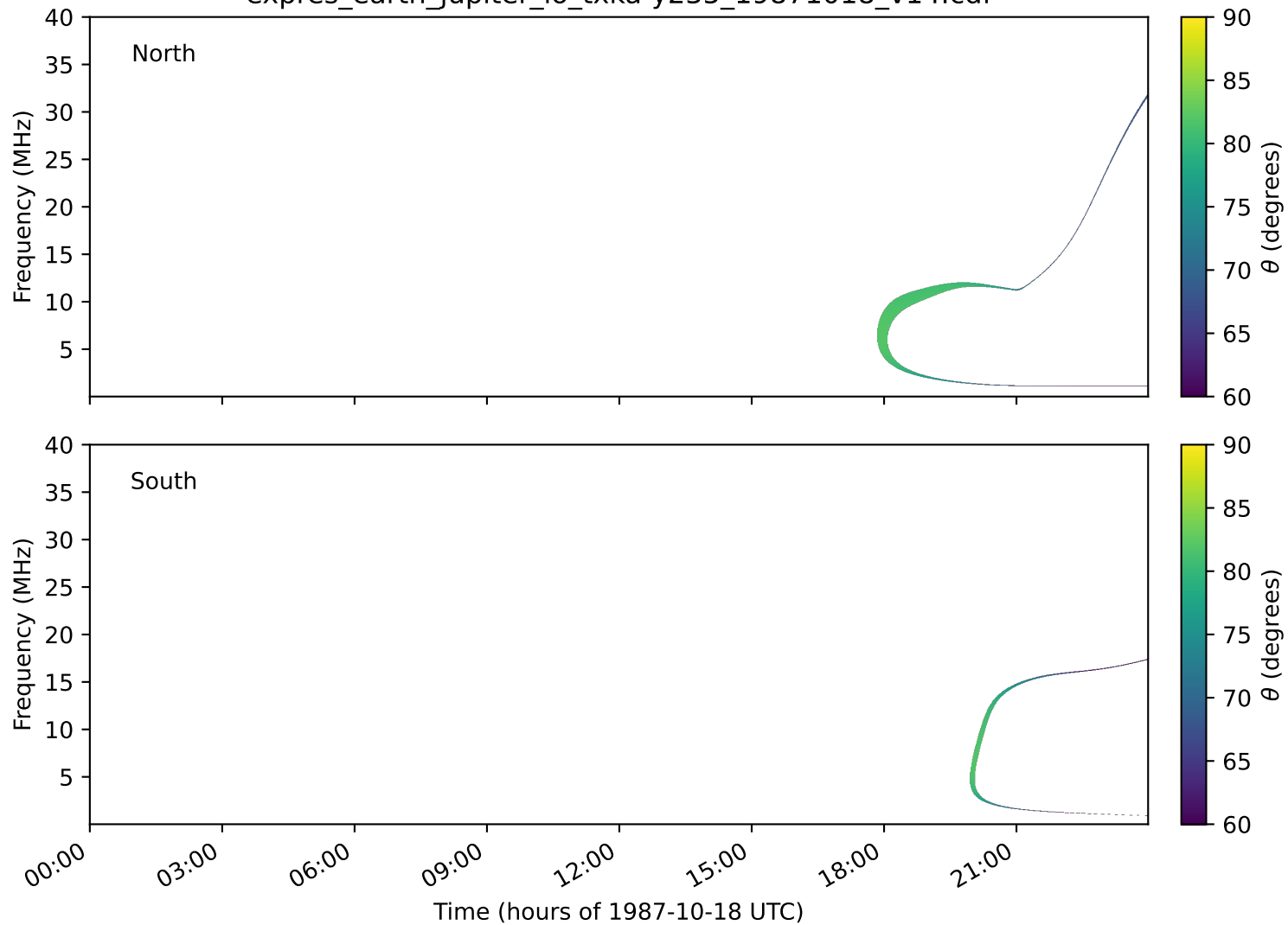
expres_earth_jupiter_io_txka-y235_19871018_v14.cdf
