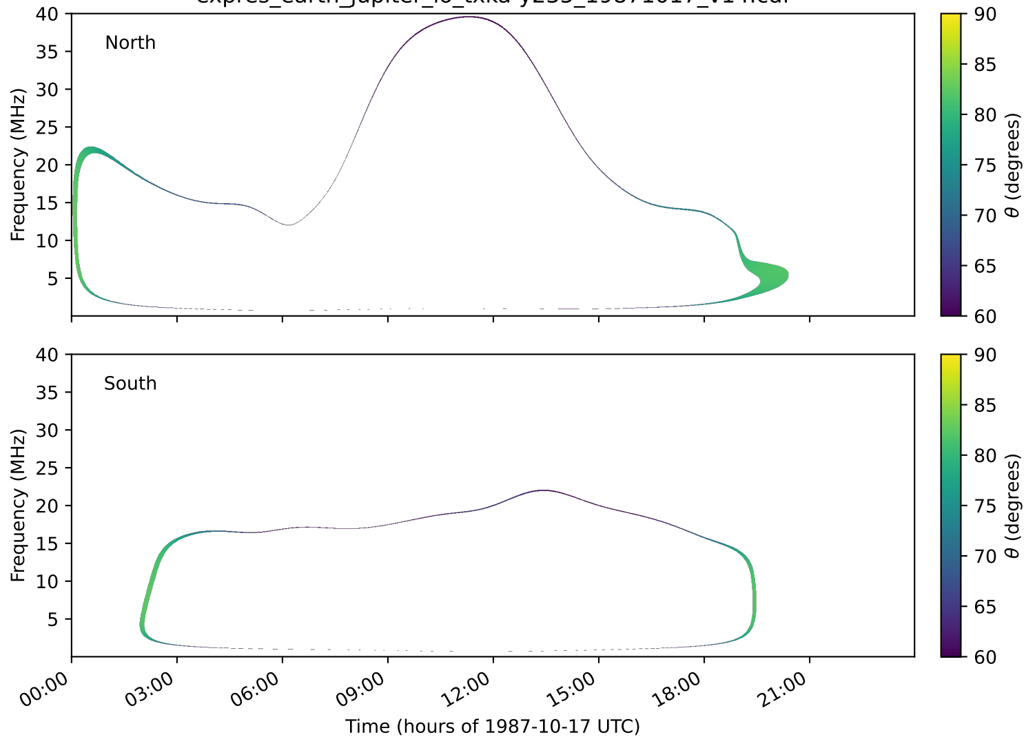
expres_earth_jupiter_io_txka-y235_19871017_v14.cdf
