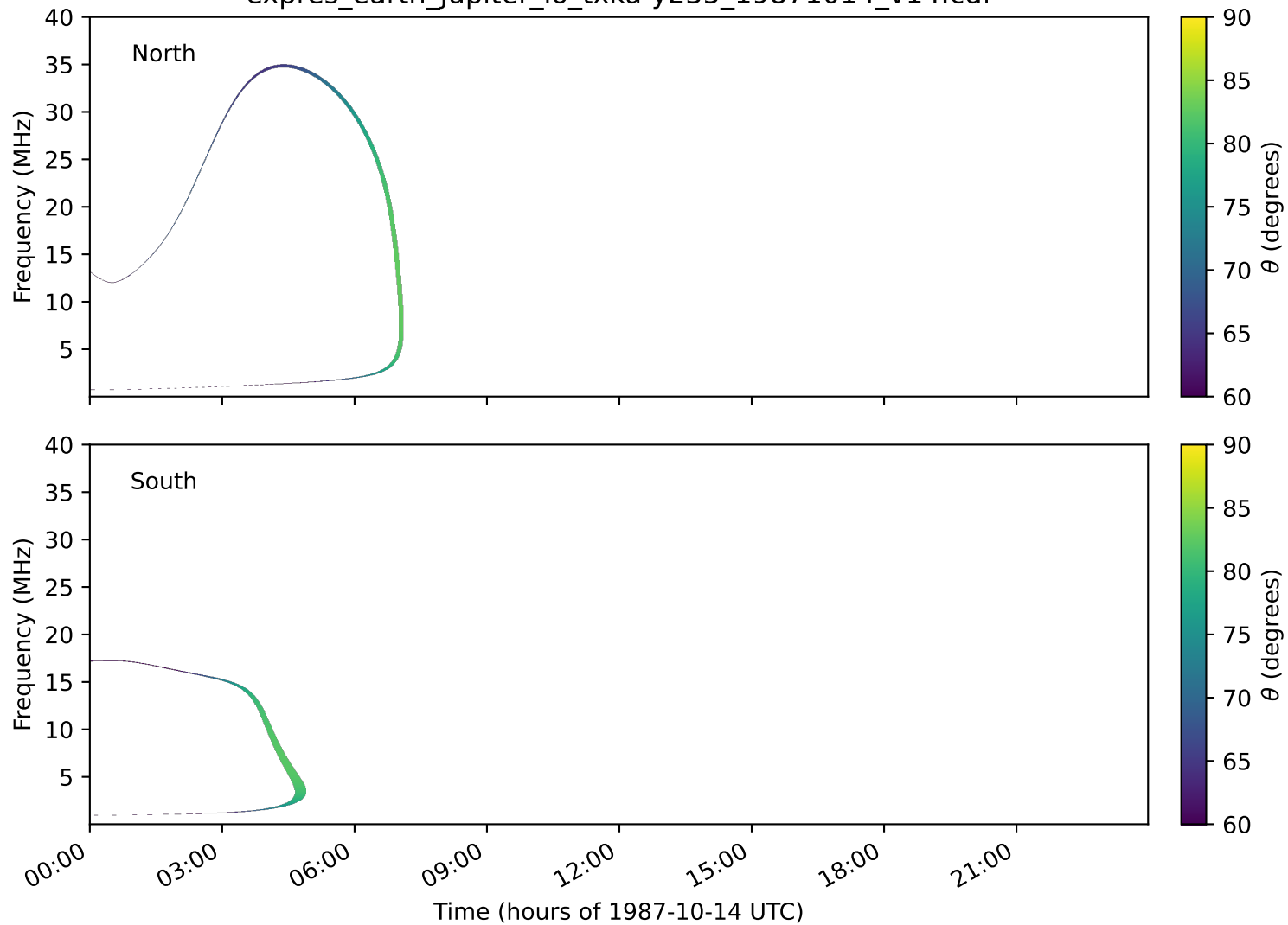
expres_earth_jupiter_io_txka-y235_19871014_v14.cdf
